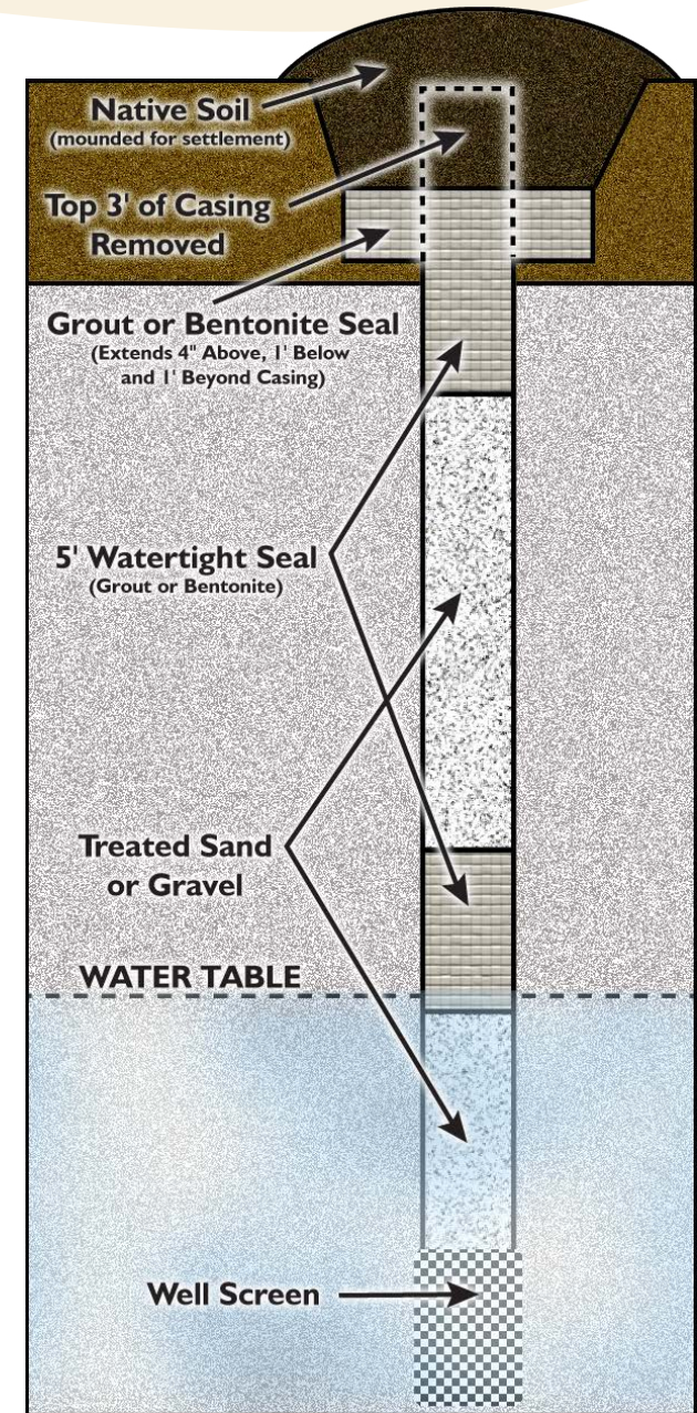
PROPERLY DECOMMISSIONED WELL (not to scale)
